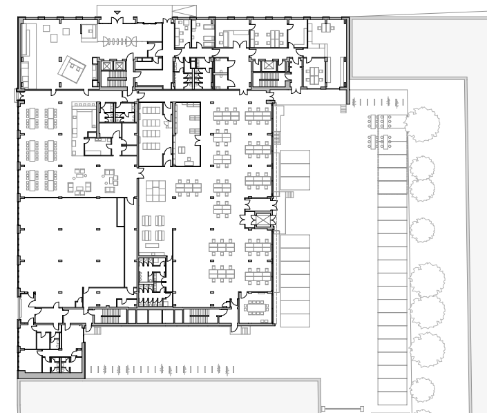
Tech Hub ground floor plan
